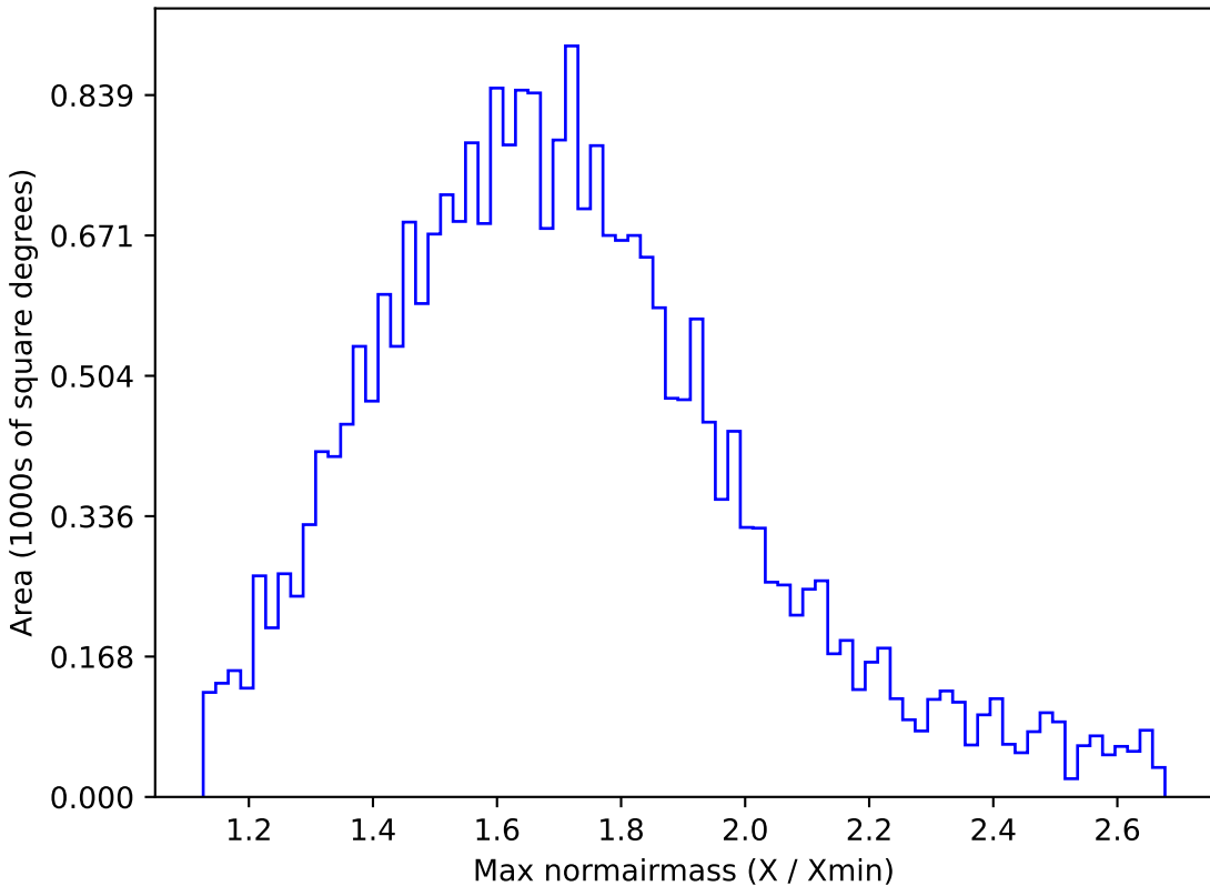
baseline_v2.0_10yrs All sky i band: Max normairmass
