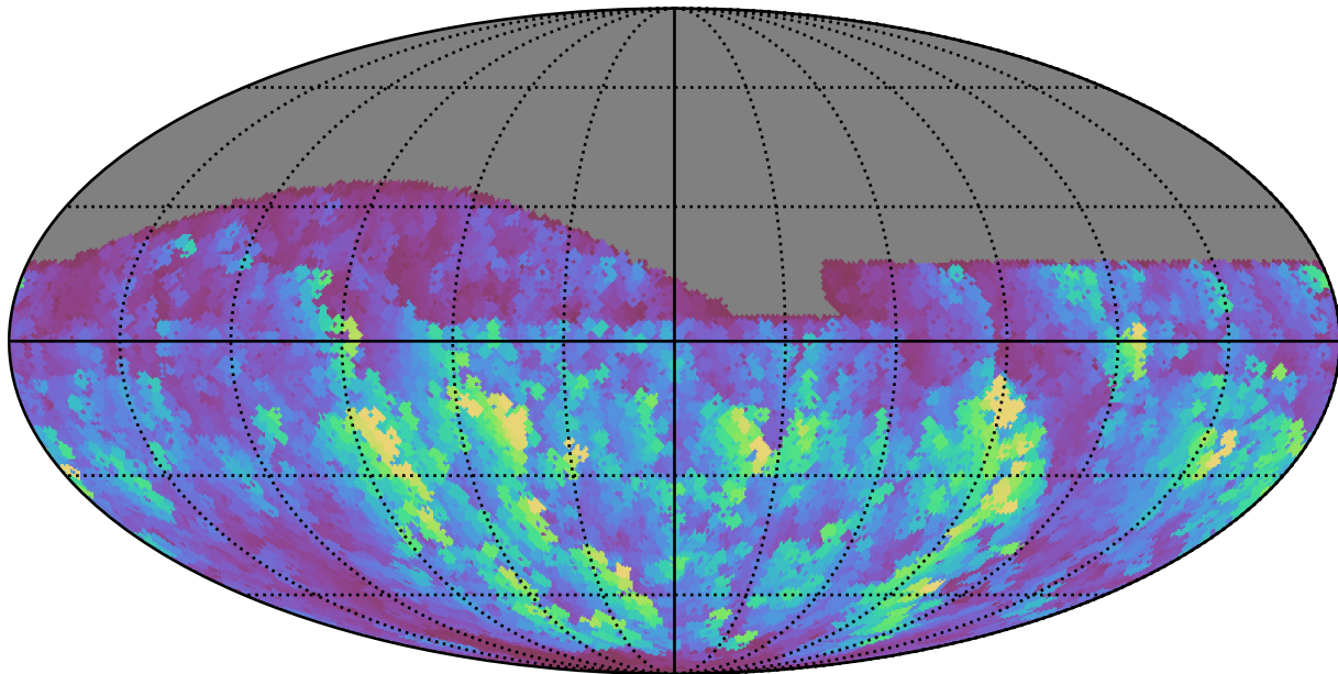
baseline_v2.0_10yrs All sky g band: Max normairmass
