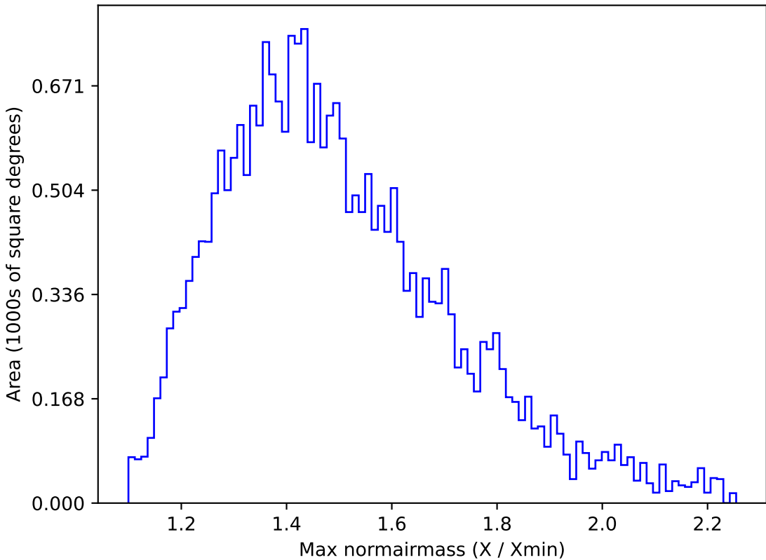
baseline_v2.0_10yrs All sky g band: Max normairmass
