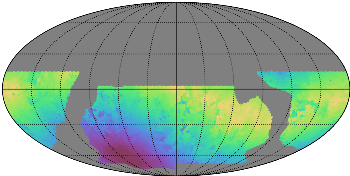
baseline_v2.0_10yrs WFD z band: Max moonDistance
