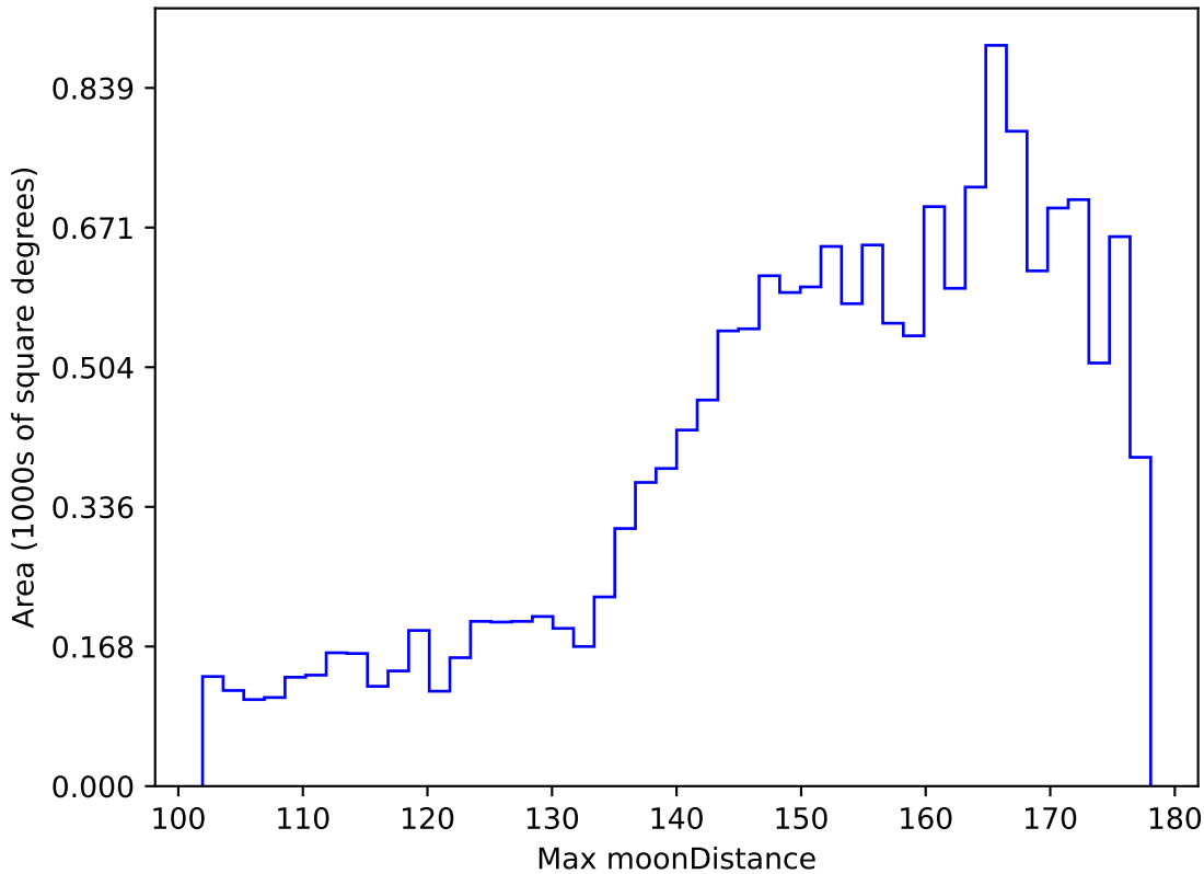
baseline_v2.0_10yrs WFD z band: Max moonDistance
