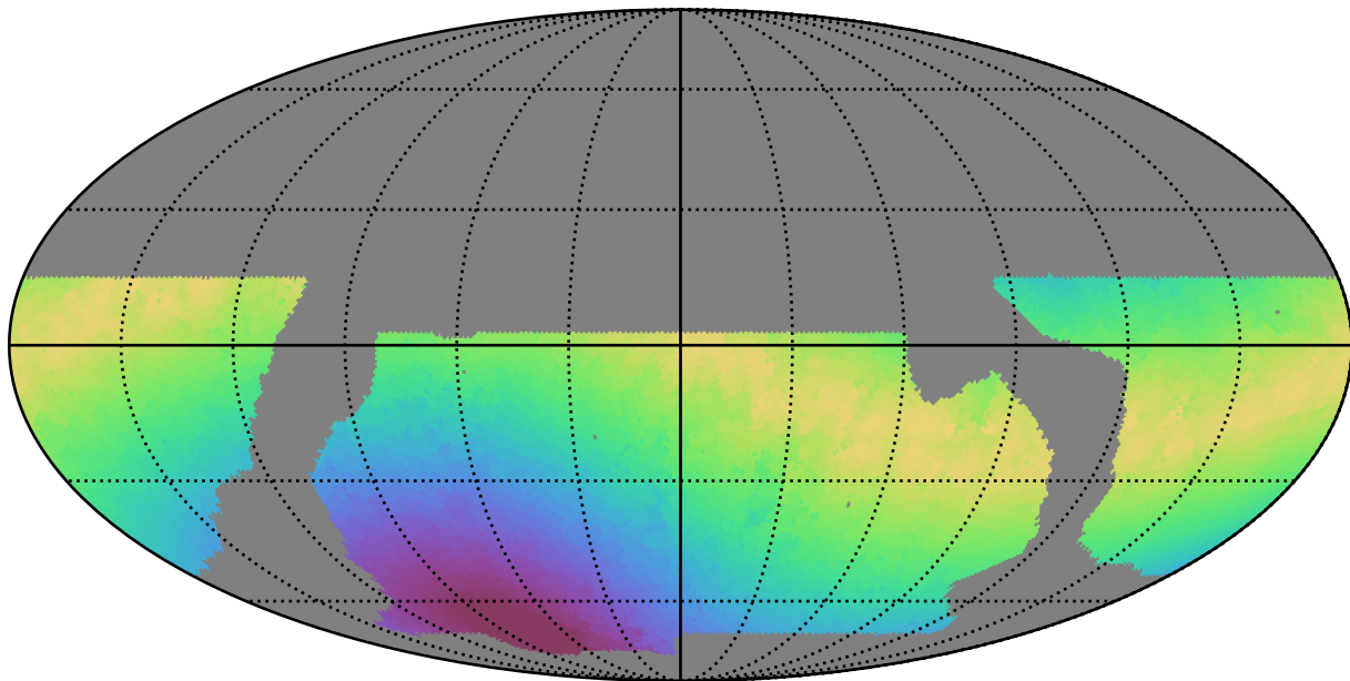
baseline_v2.0_10yrs WFD u band: Max moonDistance
