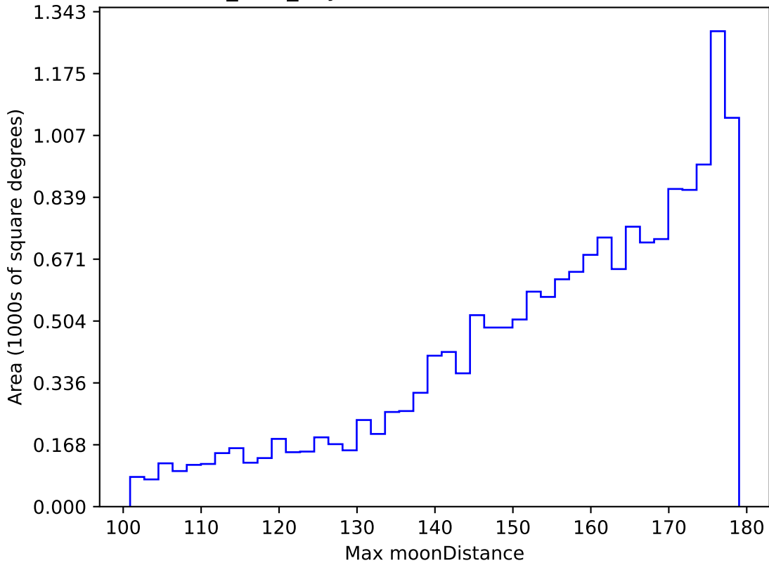
baseline_v2.0_10yrs WFD u band: Max moonDistance
