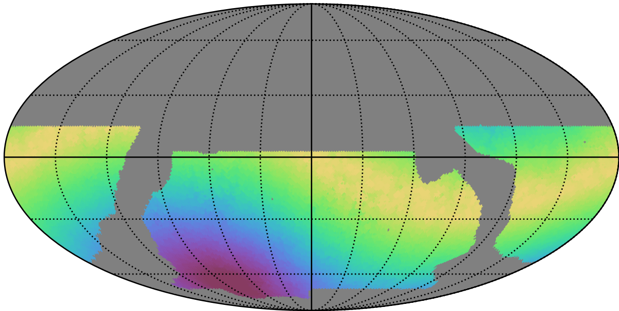
baseline_v2.0_10yrs WFD r band: Max moonDistance
