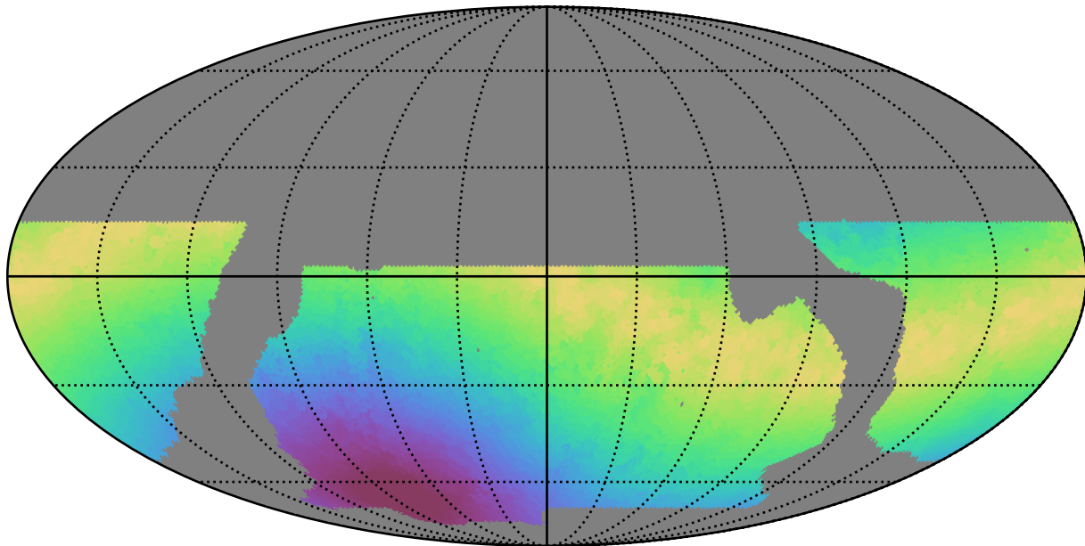
baseline_v2.0_10yrs WFD i band: Max moonDistance
