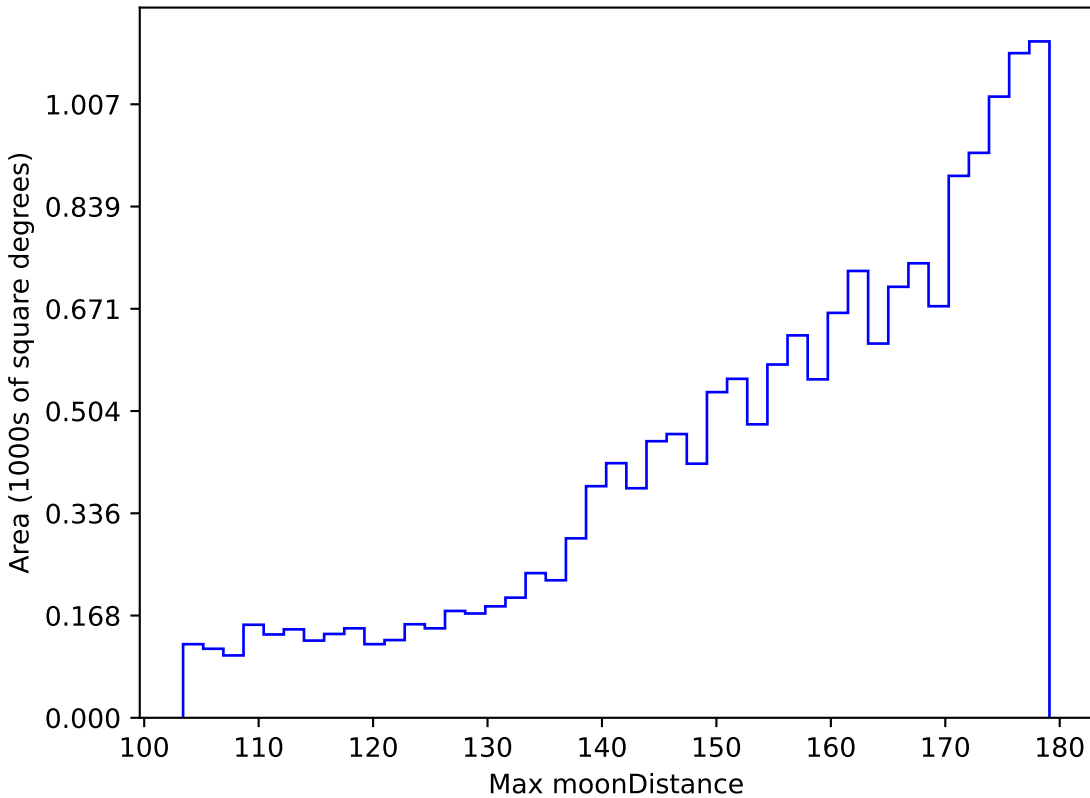
baseline_v2.0_10yrs WFD i band: Max moonDistance
