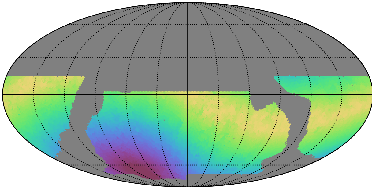
baseline_v2.0_10yrs WFD g band: Max moonDistance
