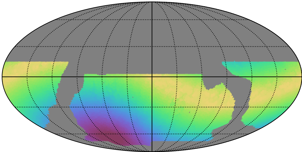
baseline_v2.0_10yrs WFD all bands: Max moonDistance
