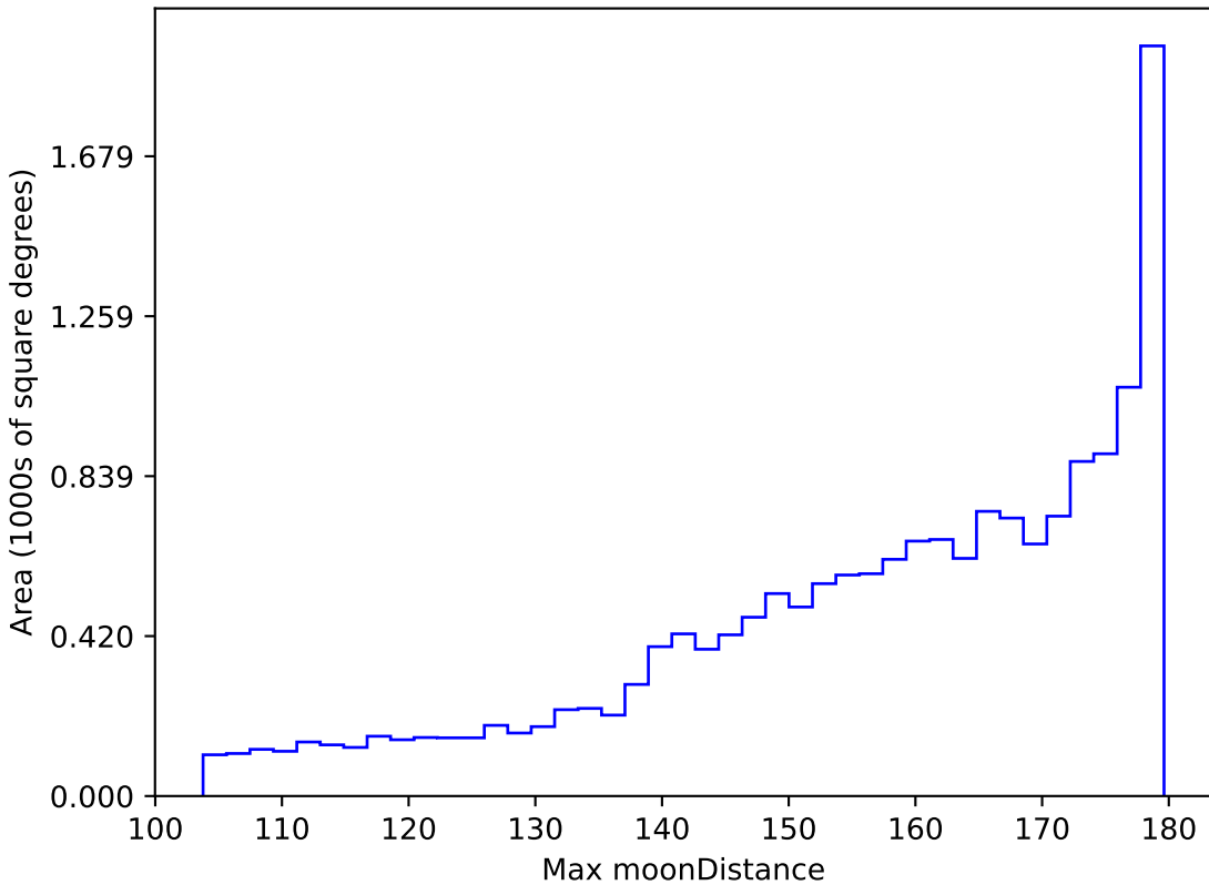
baseline_v2.0_10yrs WFD all bands: Max moonDistance
