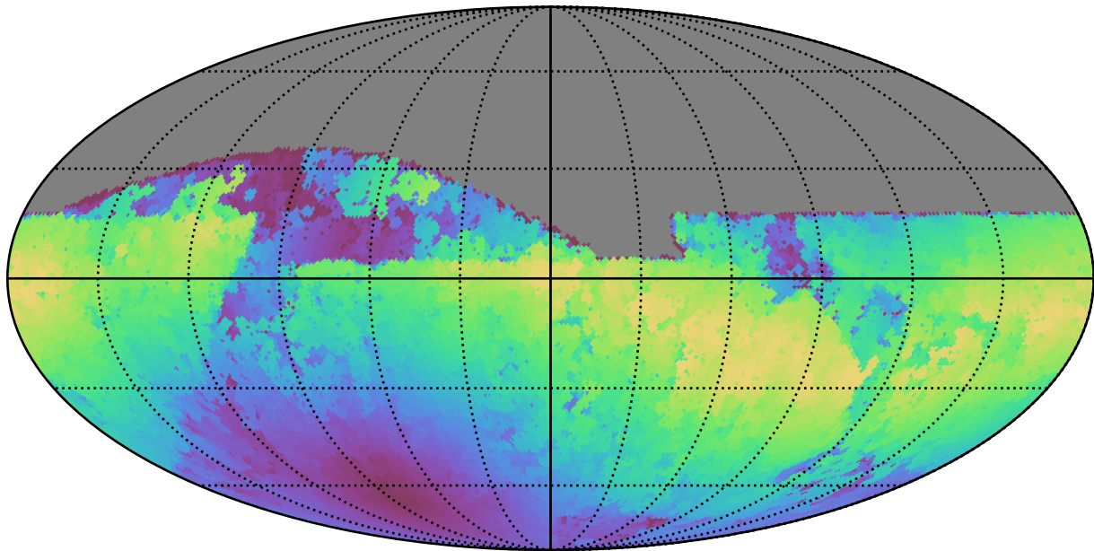
baseline_v2.0_10yrs All sky z band: Max moonDistance
