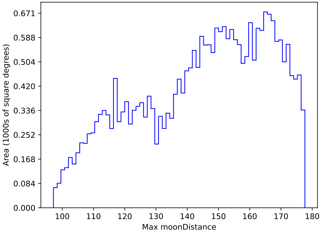
baseline_v2.0_10yrs All sky z band: Max moonDistance
