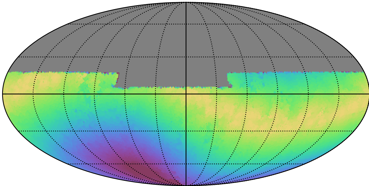
baseline_v2.0_10yrs All sky u band: Max moonDistance
