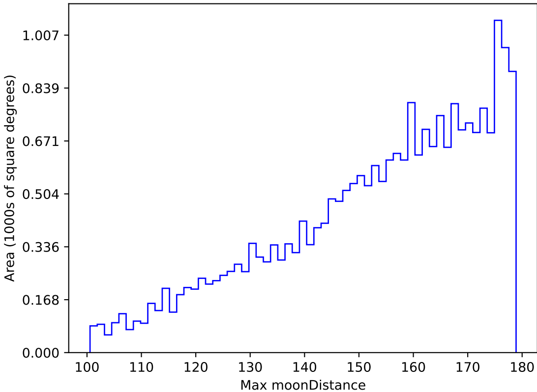
baseline_v2.0_10yrs All sky u band: Max moonDistance
