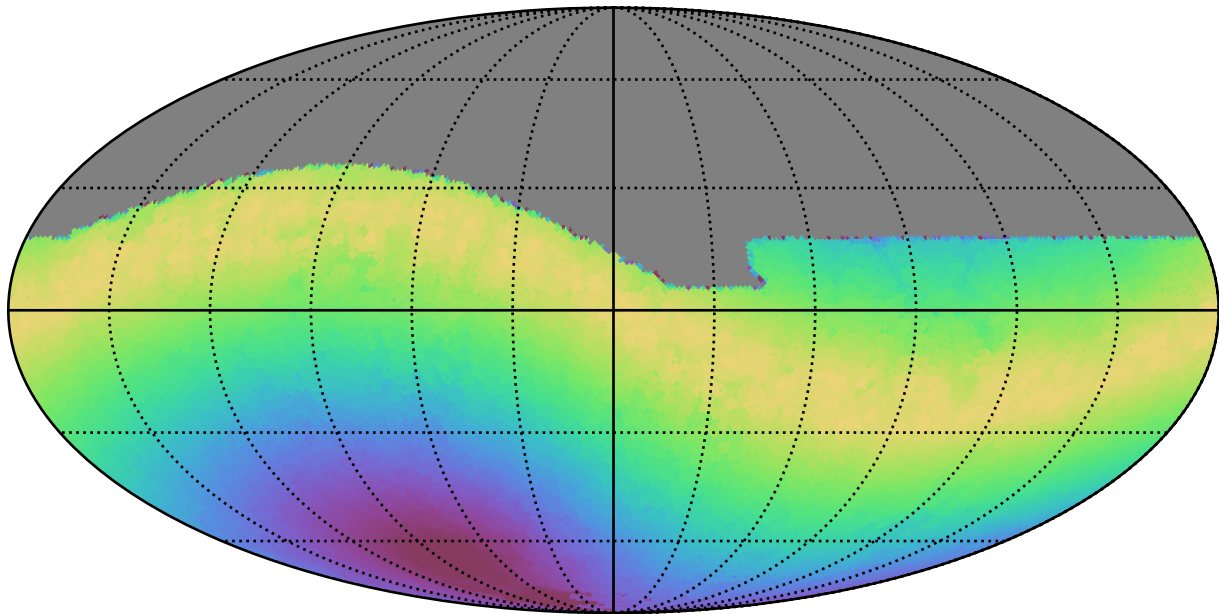
baseline_v2.0_10yrs All sky r band: Max moonDistance
