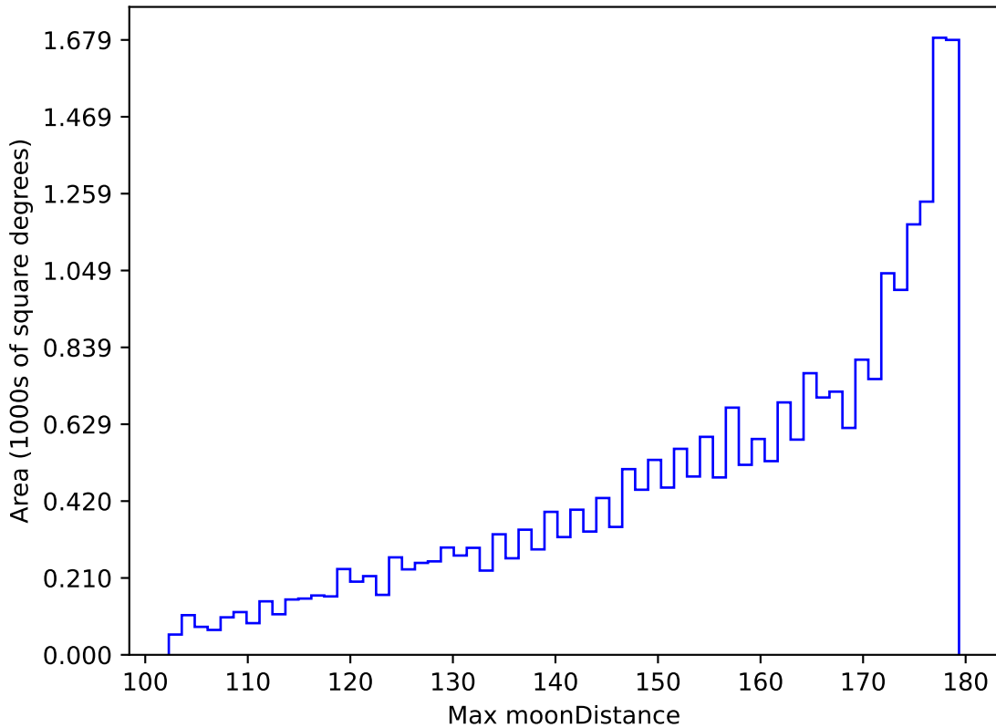
baseline_v2.0_10yrs All sky r band: Max moonDistance
