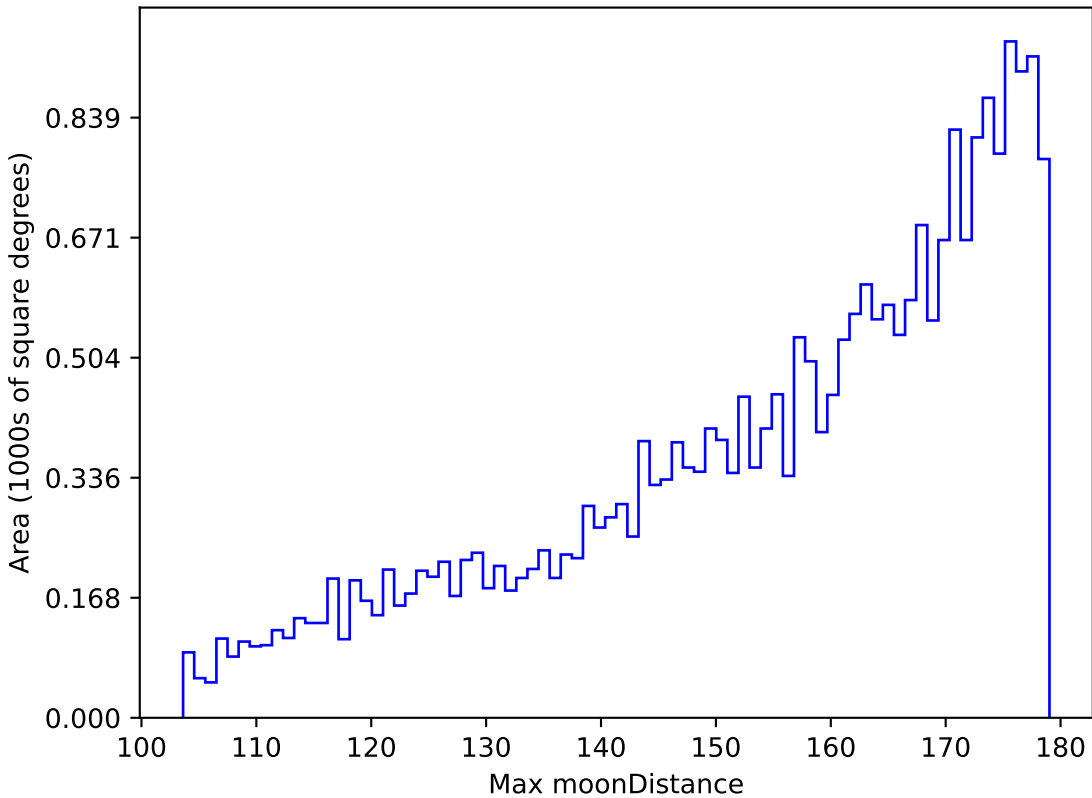
baseline_v2.0_10yrs All sky i band: Max moonDistance
