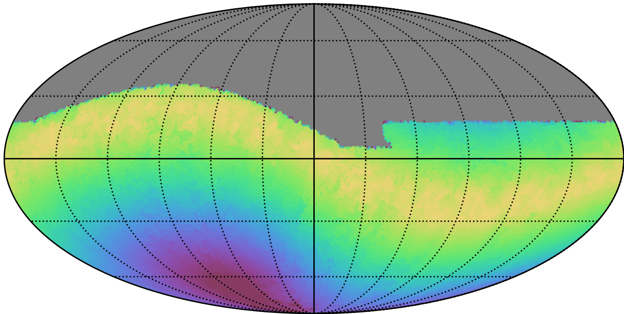
baseline_v2.0_10yrs All sky g band: Max moonDistance
