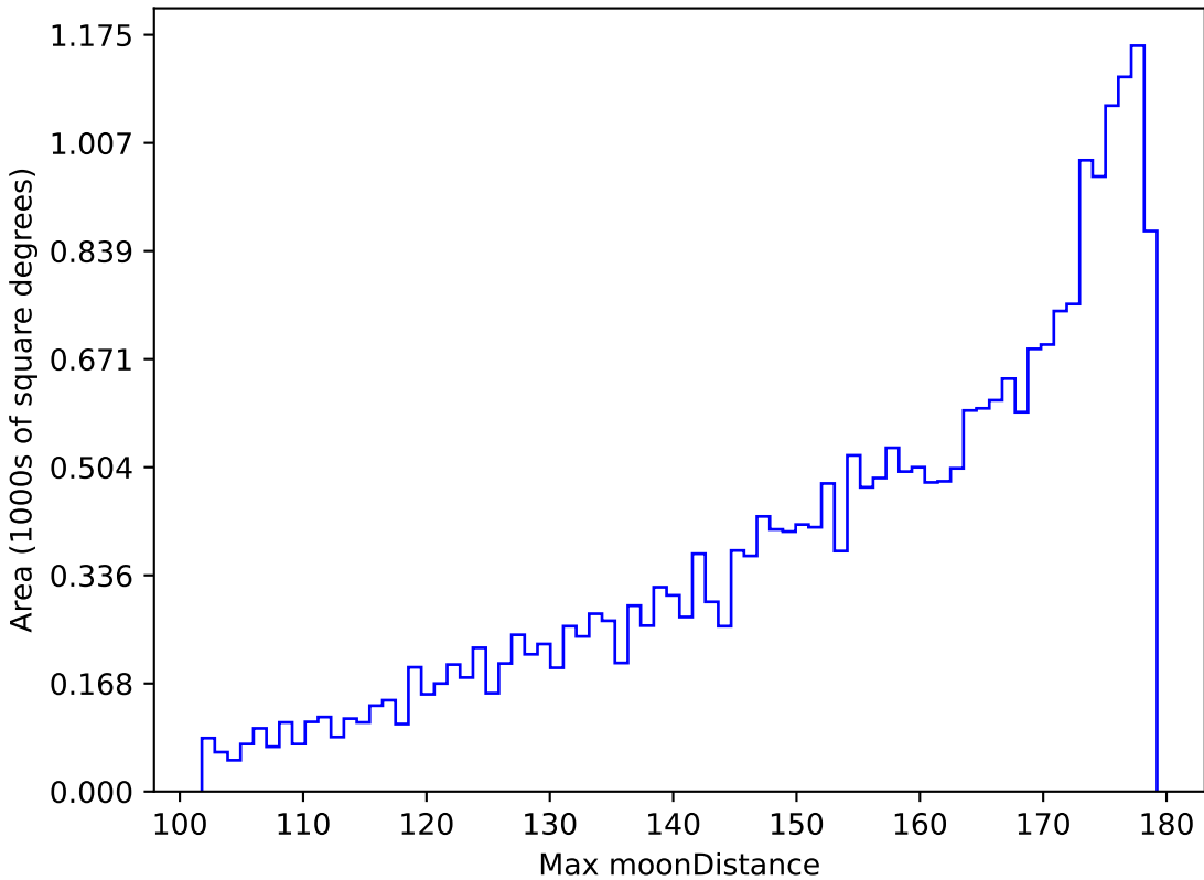
baseline_v2.0_10yrs All sky g band: Max moonDistance
