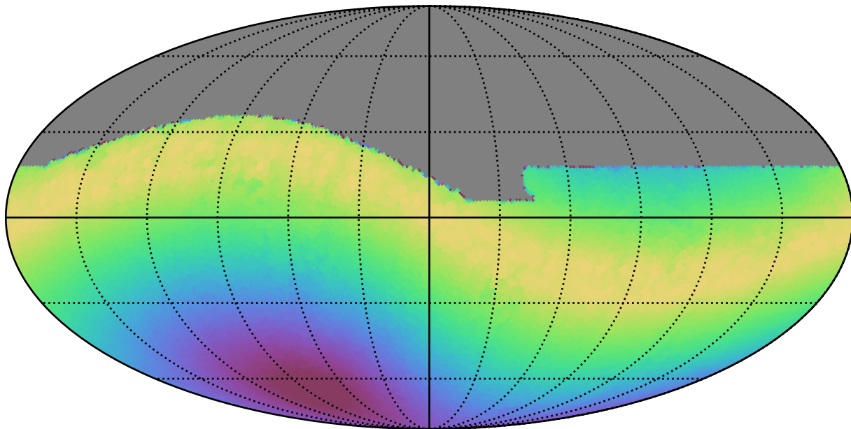
baseline_v2.0_10yrs All sky all bands: Max moonDistance
