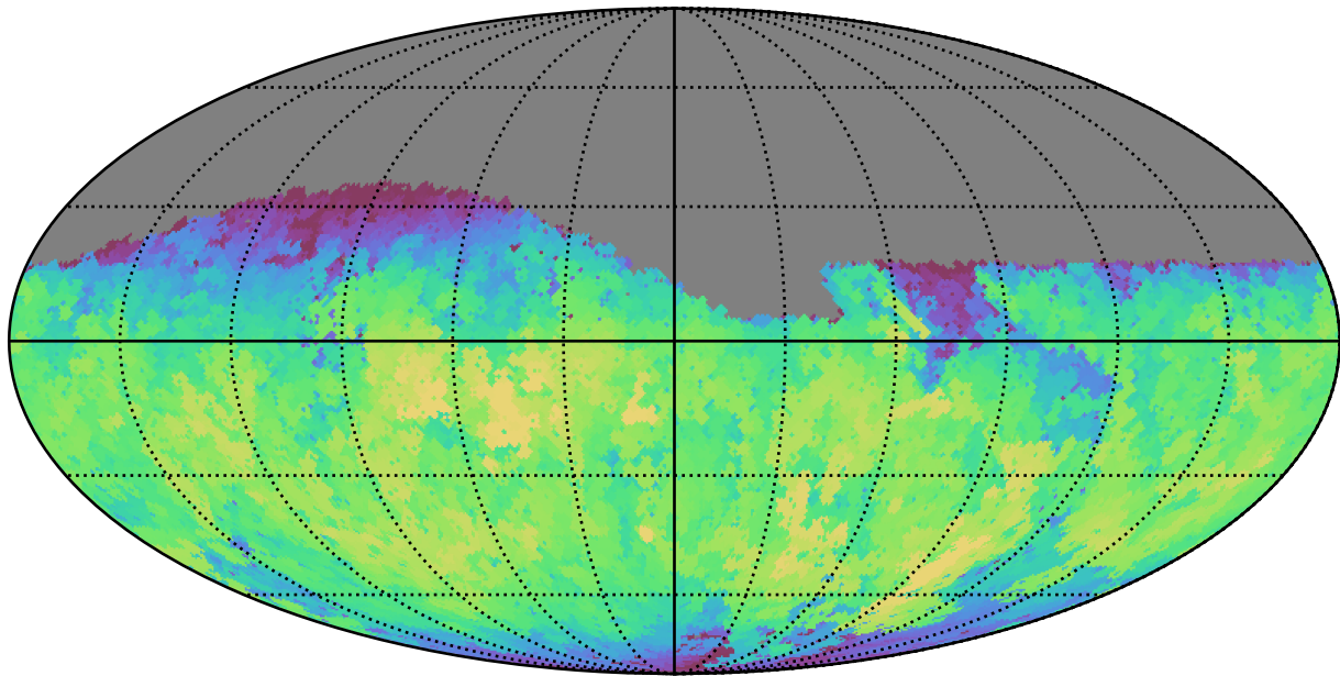
baseline_v2.0_10yrs Yr 1 z band: Max fiveSigmaDepth
