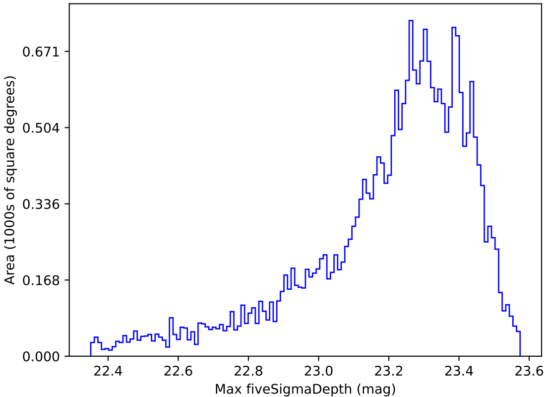
baseline_v2.0_10yrs Yr 1 z band: Max fiveSigmaDepth
