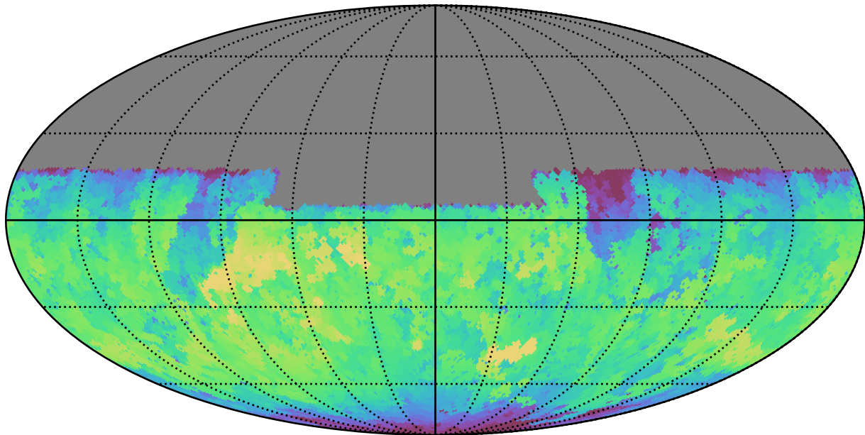
baseline_v2.0_10yrs Yr 1 y band: Max fiveSigmaDepth
