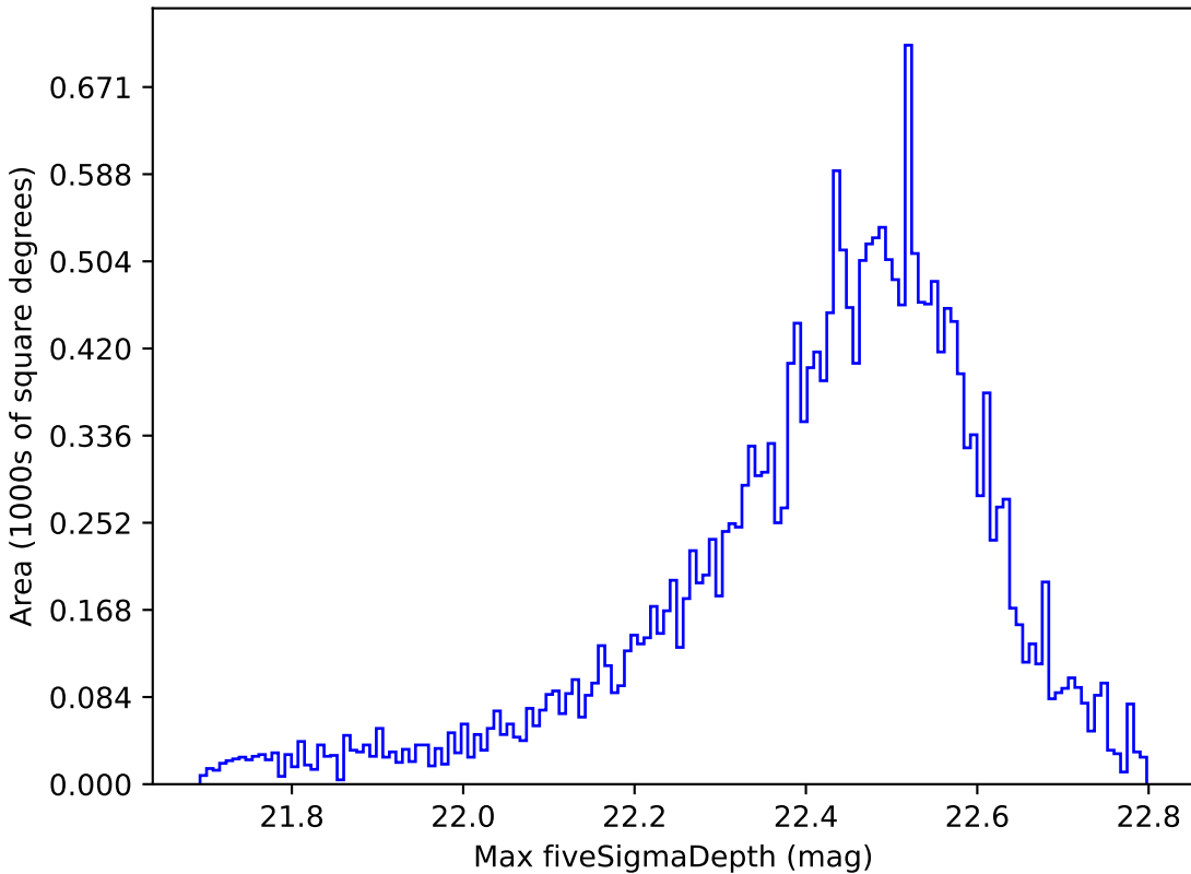
baseline_v2.0_10yrs Yr 1 y band: Max fiveSigmaDepth
