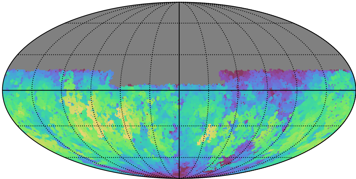
baseline_v2.0_10yrs Yr 1 u band: Max fiveSigmaDepth
