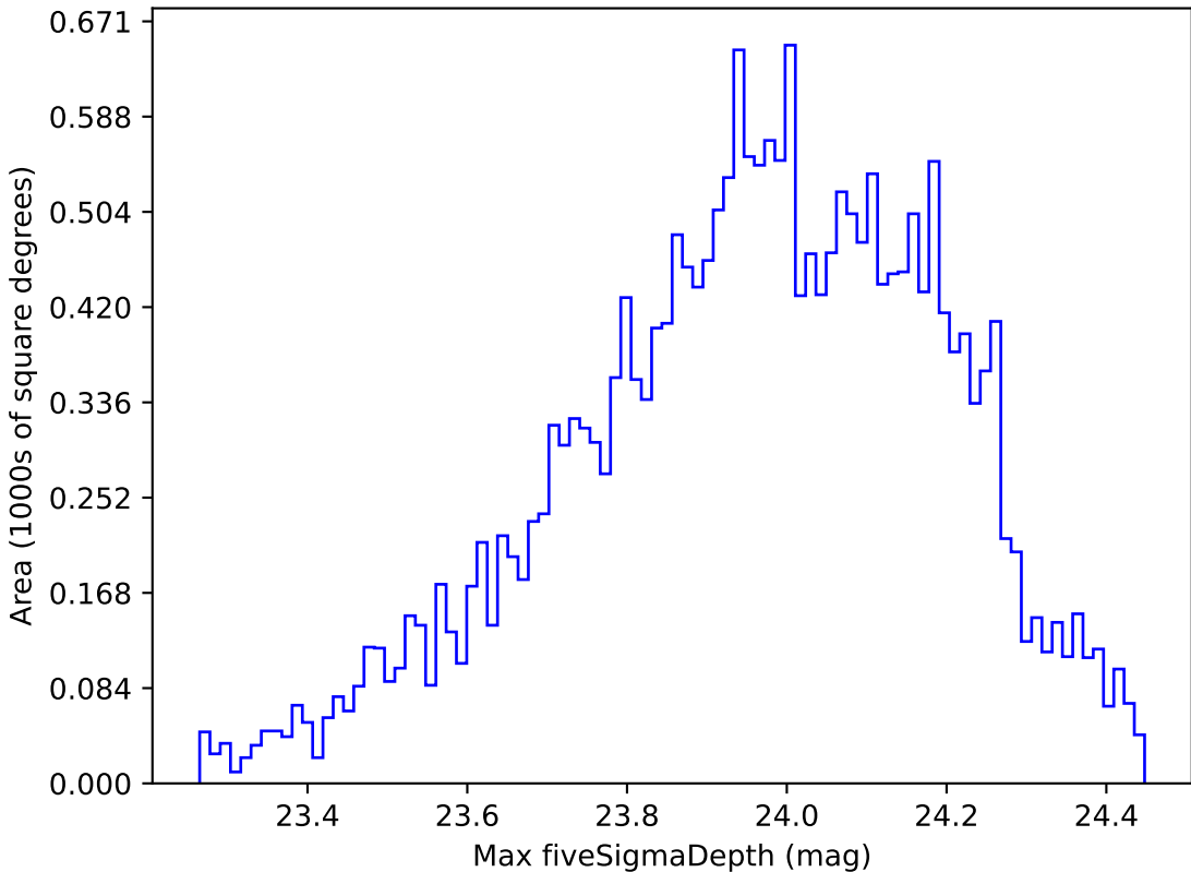
baseline_v2.0_10yrs Yr 1 u band: Max fiveSigmaDepth
