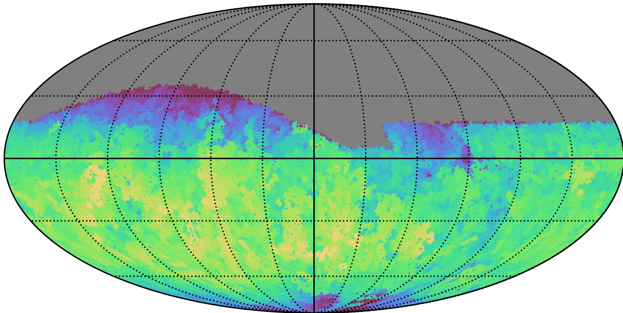
baseline_v2.0_10yrs Yr 1 r band: Max fiveSigmaDepth
