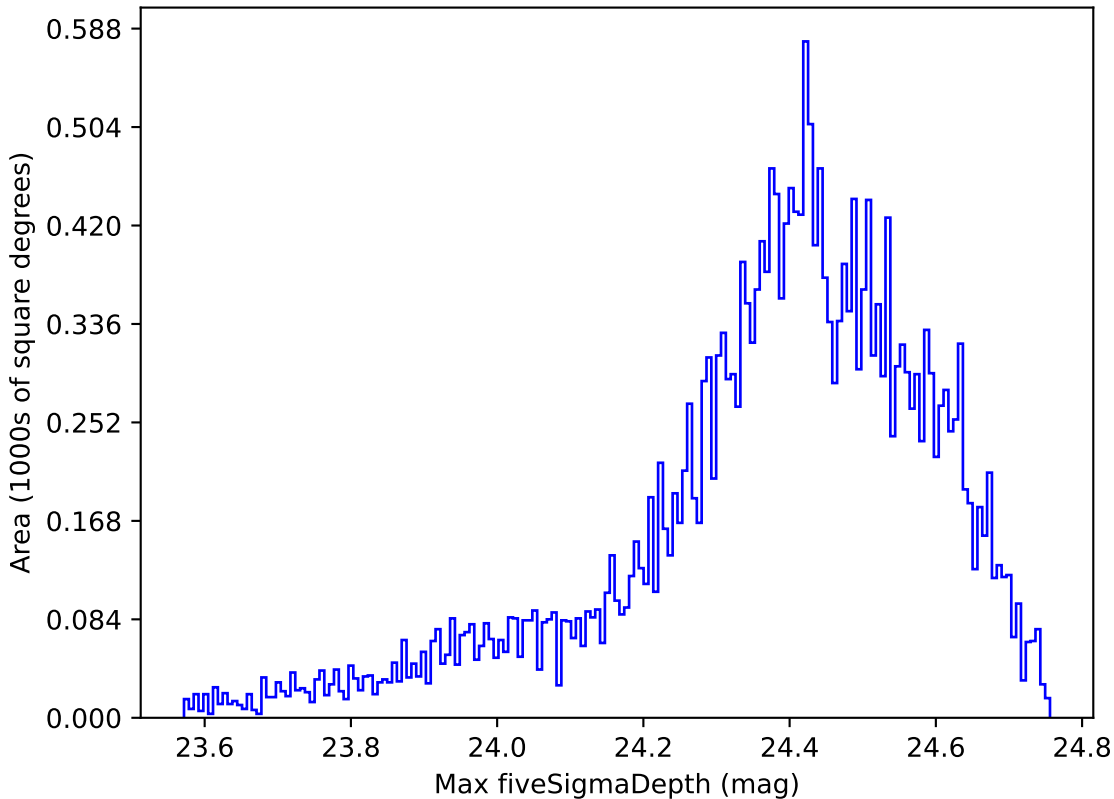
baseline_v2.0_10yrs Yr 1 r band: Max fiveSigmaDepth
