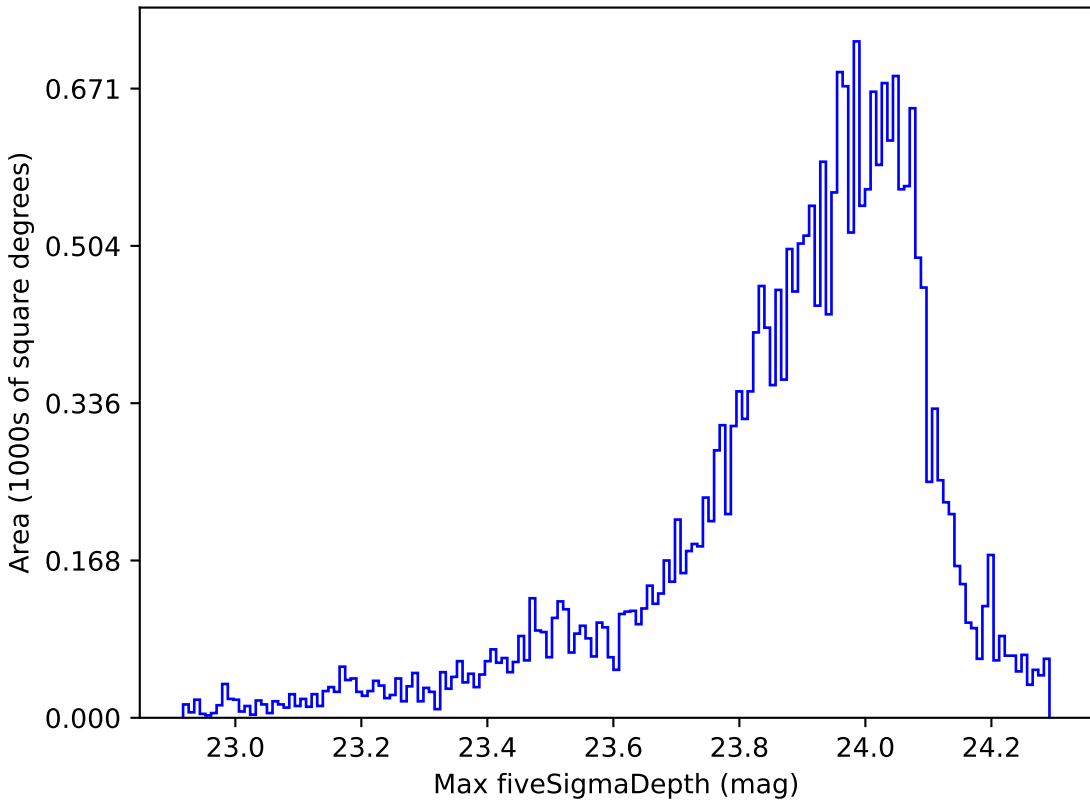
baseline_v2.0_10yrs Yr 1 i band: Max fiveSigmaDepth
