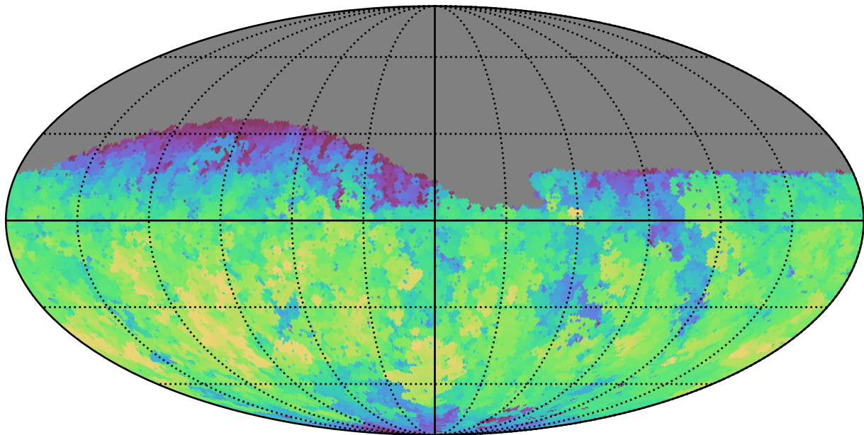
baseline_v2.0_10yrs Yr 1 g band: Max fiveSigmaDepth
