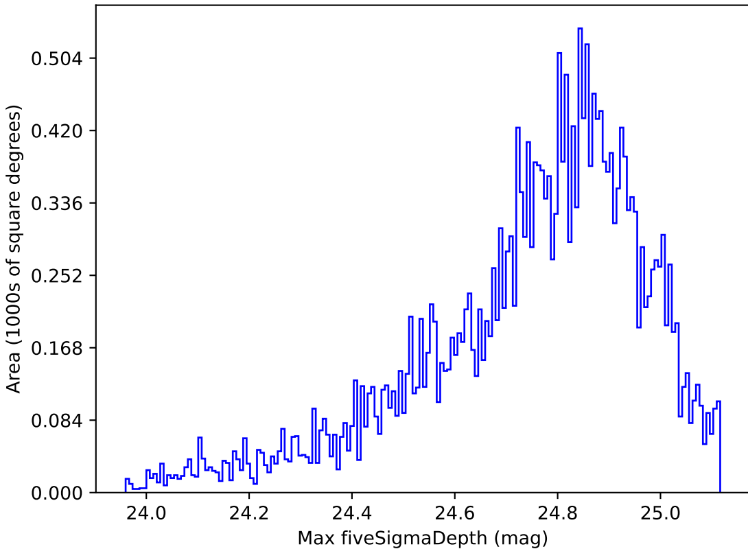
baseline_v2.0_10yrs Yr 1 g band: Max fiveSigmaDepth
