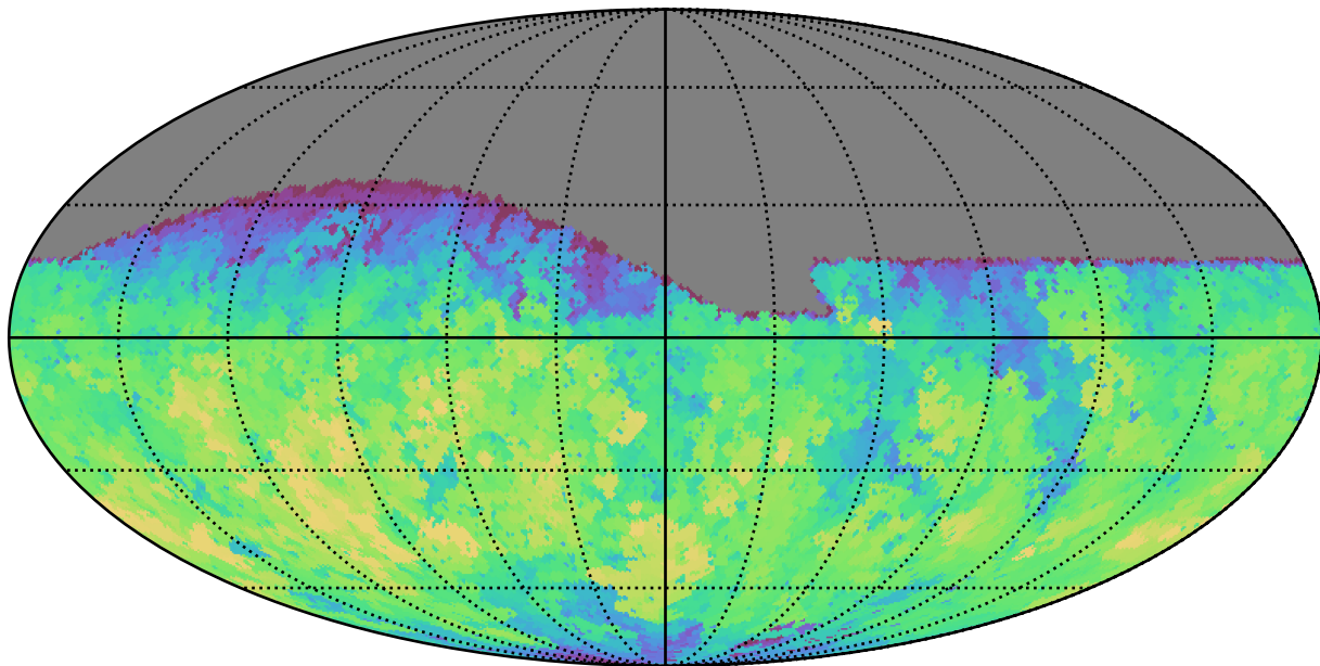
baseline_v2.0_10yrs Yr 1 all bands: Max fiveSigmaDepth
