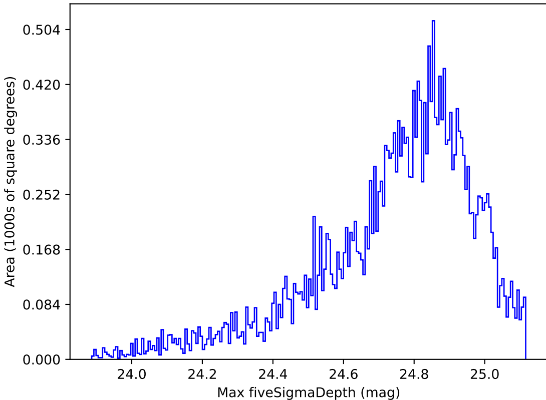
baseline_v2.0_10yrs Yr 1 all bands: Max fiveSigmaDepth
