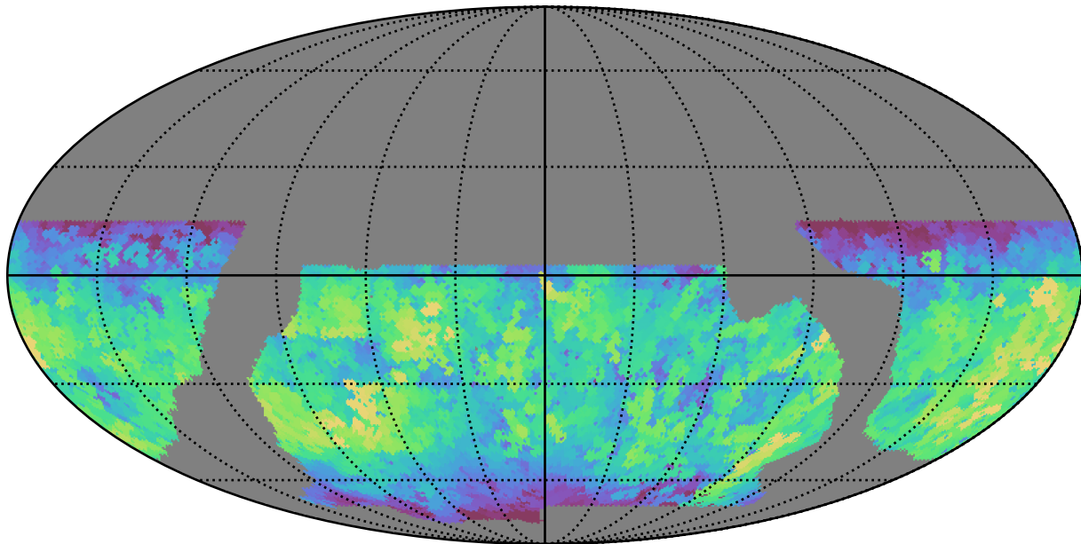
baseline_v2.0_10yrs WFD z band: Max fiveSigmaDepth
