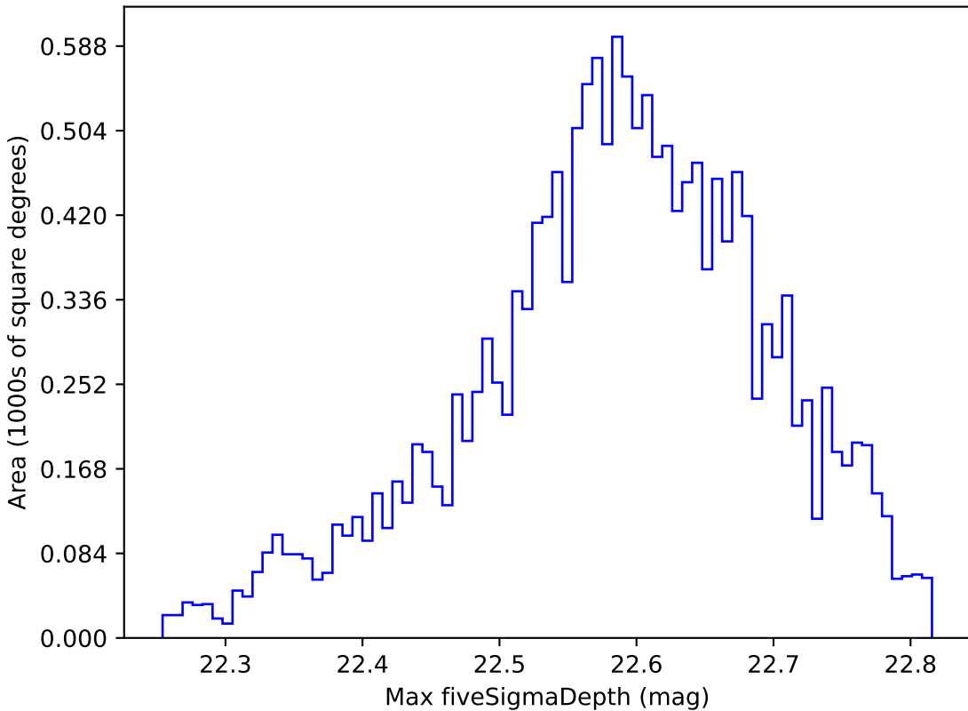
baseline_v2.0_10yrs WFD y band: Max fiveSigmaDepth
