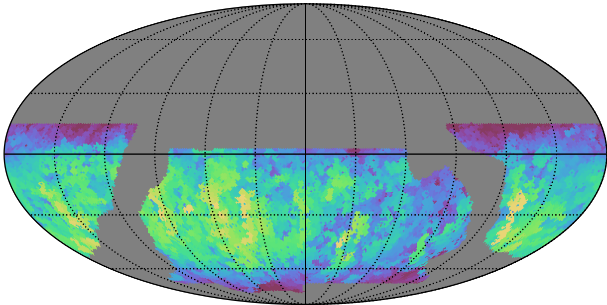
baseline_v2.0_10yrs WFD u band: Max fiveSigmaDepth
