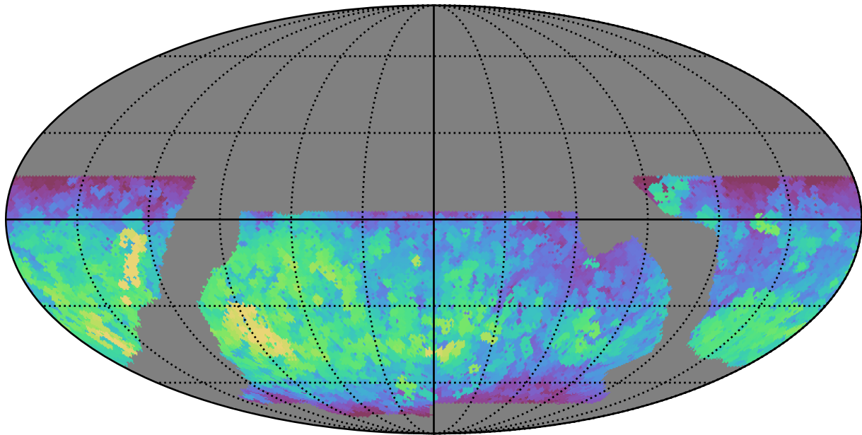
baseline_v2.0_10yrs WFD r band: Max fiveSigmaDepth
