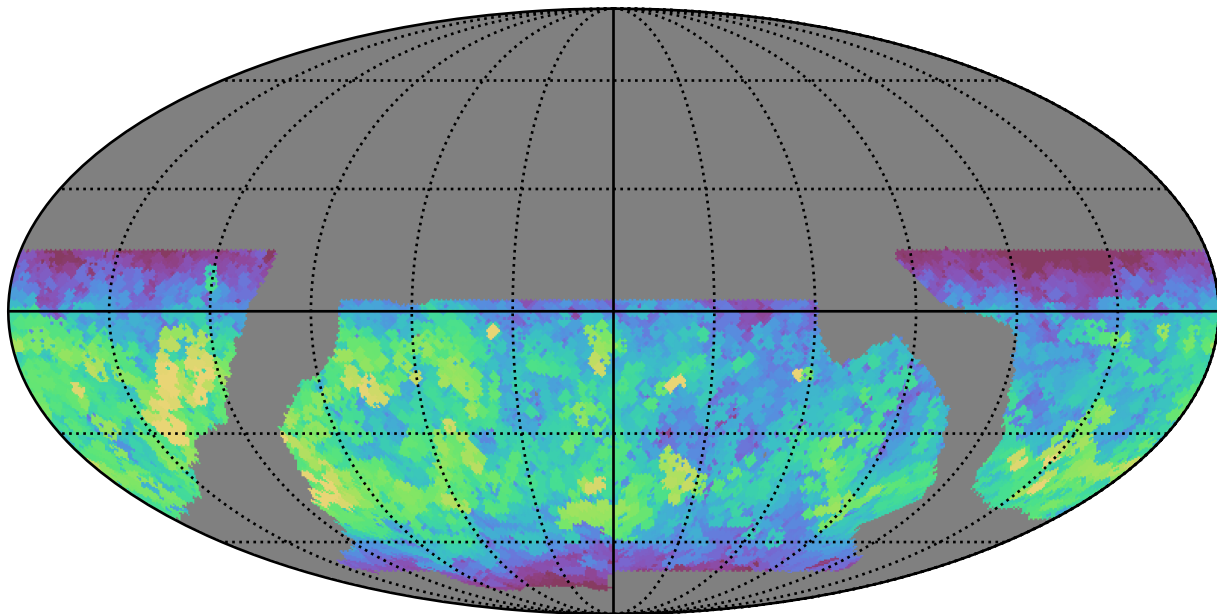
baseline_v2.0_10yrs WFD i band: Max fiveSigmaDepth
