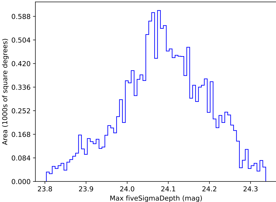
baseline_v2.0_10yrs WFD i band: Max fiveSigmaDepth
