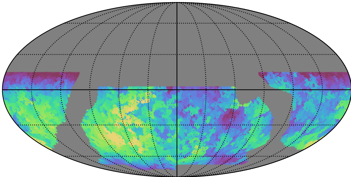
baseline_v2.0_10yrs WFD g band: Max fiveSigmaDepth
