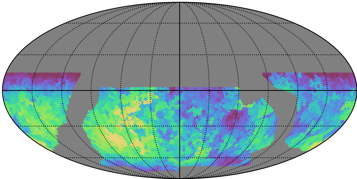
baseline_v2.0_10yrs WFD all bands: Max fiveSigmaDepth
