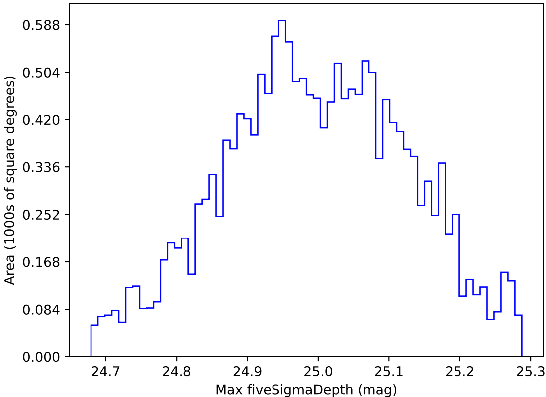
baseline_v2.0_10yrs WFD all bands: Max fiveSigmaDepth
