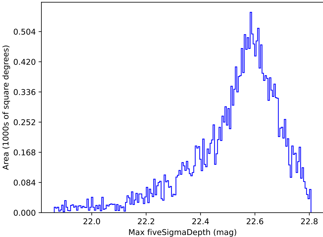
baseline_v2.0_10yrs All sky y band: Max fiveSigmaDepth
