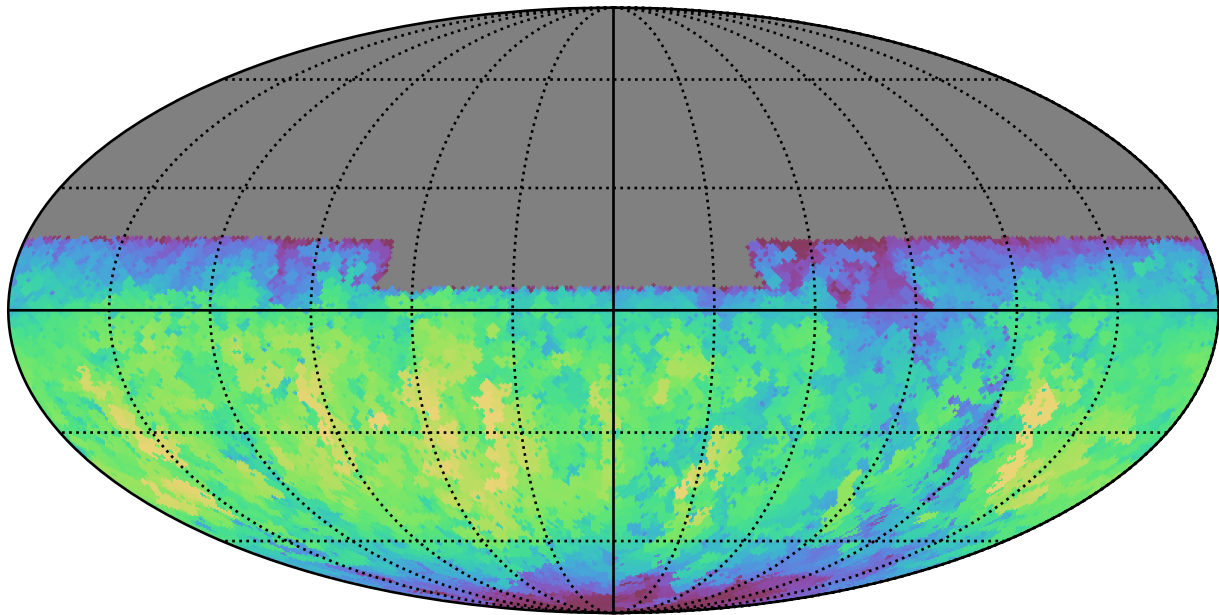
baseline_v2.0_10yrs All sky u band: Max fiveSigmaDepth
