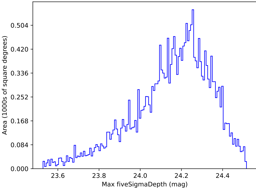
baseline_v2.0_10yrs All sky u band: Max fiveSigmaDepth
