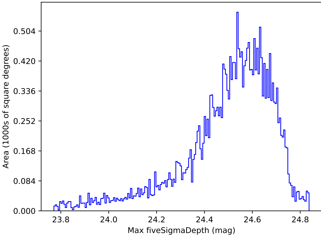
baseline_v2.0_10yrs All sky r band: Max fiveSigmaDepth
