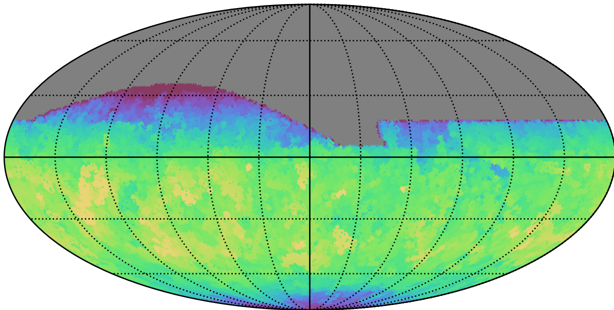
baseline_v2.0_10yrs All sky i band: Max fiveSigmaDepth
